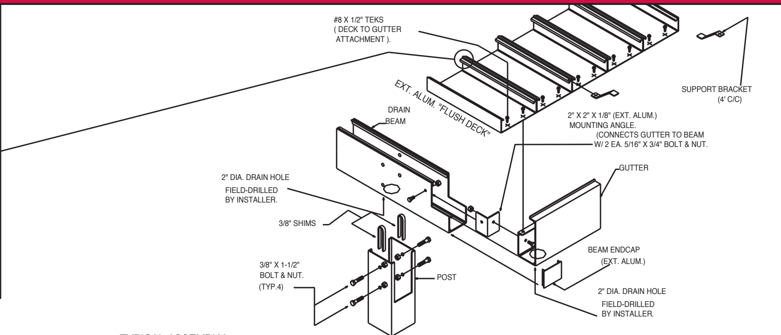
TYPICAL ASSEMBLY (CANOPY TOP)
