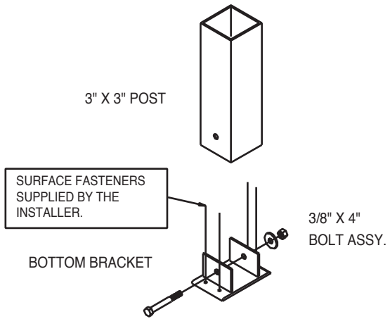
TYPICAL SURFACE-MOUNT ( 3" X 3" POST ) ( USED ON WALL-ATTACHED CANOPIES ONLY )
